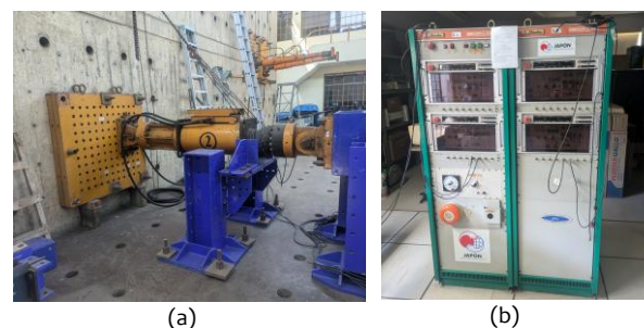
Fig. 1. The CISMID's Laboratory Actuator system: (a) Servo-hydraulic actuator, (b) Servo-controller.
