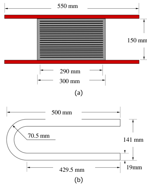
Fig. 7. ABC-RU specimen dimensions: (a) Rubber bearing, (b) U-shaped steel damper [15].
